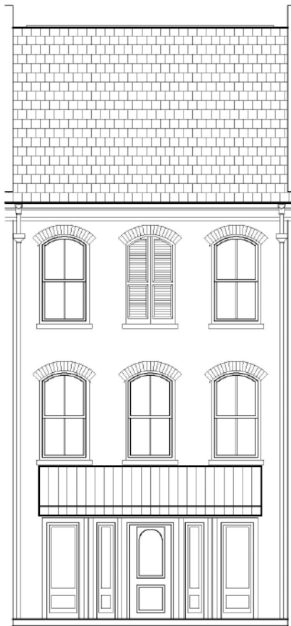
Elevation - One
